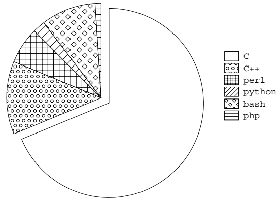
Figure 2. Language repartition of vulnerabilities in open source softwares as reported by Debian Security in 2005
