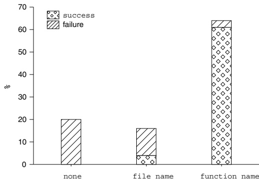
Figure 4. Success to locate vulnerabilities depending on information provided
