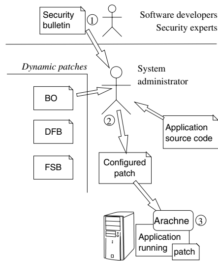
Figure 1. Workflow of dynamic patching
