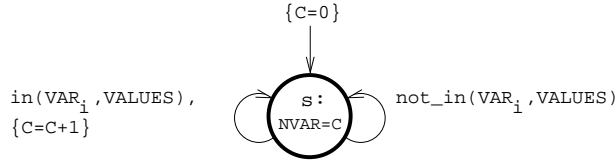
Figure 5.23: Automaton (with a counter) of the among constraint
