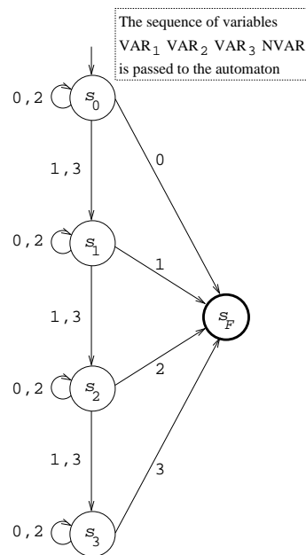
Figure 5.25: Counter free non deterministic automaton of the \text{among}(NVAR, \langle VAR_1, VAR_2, VAR_3 \rangle, \langle 1, 3 \rangle) constraint assuming VAR_i \in [0, 3] ( 1 \leq i \leq 3 ), with initial state s_0 and final state s_F
