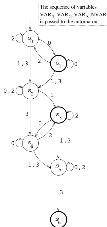
Figure 5.26: Counter free minimum-state deterministic automaton of the \text{among}(NVAR, \langle VAR_1, VAR_2, VAR_3 \rangle, \langle 1, 3 \rangle) constraint assuming VAR_i \in [0, 3] ( 1 \leq i \leq 3 ), with initial state s_0 and final state s_F
