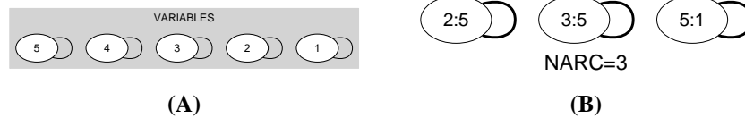
Figure 5.22: Initial and final graph of the among constraint
