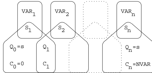
Figure 5.24: Hypergraph of the reformulation corresponding to the automaton (with a counter) of the among constraint: since all states variables are fixed to the unique state of the automaton, the transitions constraints share at most one variable and the constraint network is Berge-acyclic
