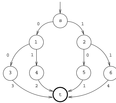
Figure 5.145: Automaton associated with the preference table of the cond_lex_lesseq constraint given in the example
