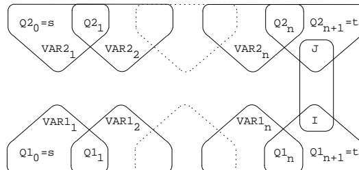
Figure 5.146: Hypergraph of the reformulation corresponding to the cond_lex_lesseq constraint: it uses two occurrences of the automaton of Figure 5.145 and the constraint I \leq J
