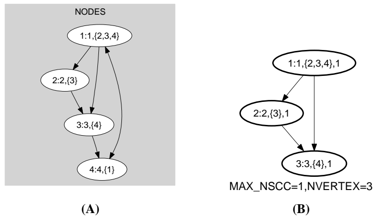
Figure 5.178: Initial and final graph of the cutset set constraint
