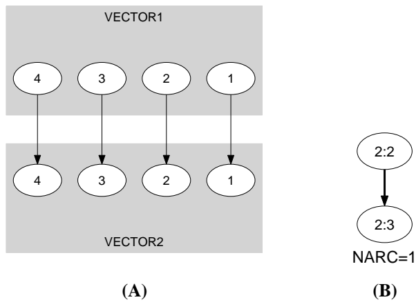
Figure 5.377: Initial and final graph of the lex_different constraint
