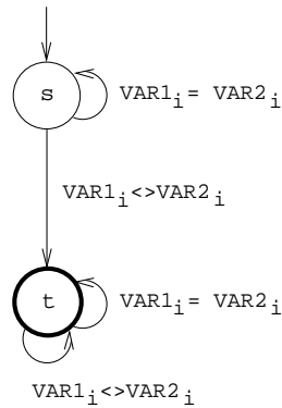
Figure 5.378: Automaton of the lex_different constraint
