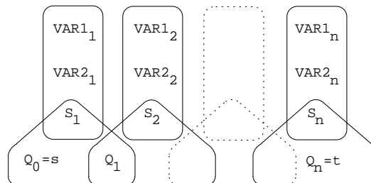
Figure 5.379: Hypergraph of the reformulation corresponding to the automaton of the lex_different constraint
