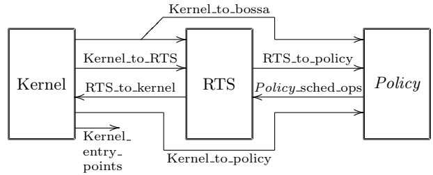
Figure 2: Bossa component structure
